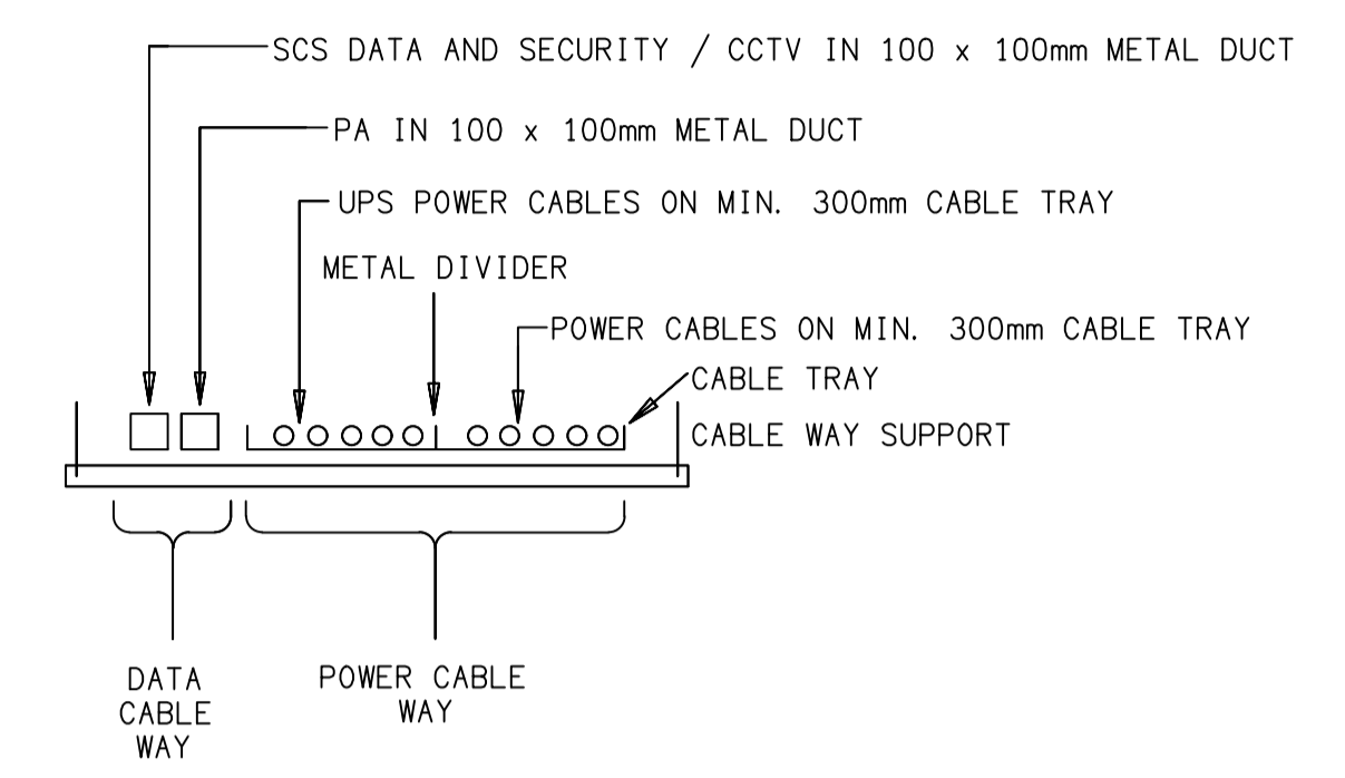
DETAIL TYPICAL MINIMUM CABLE WAY NOT TO SCALE
